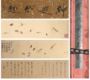
334: The Chinese painting of insects, Qi Baishi mark
